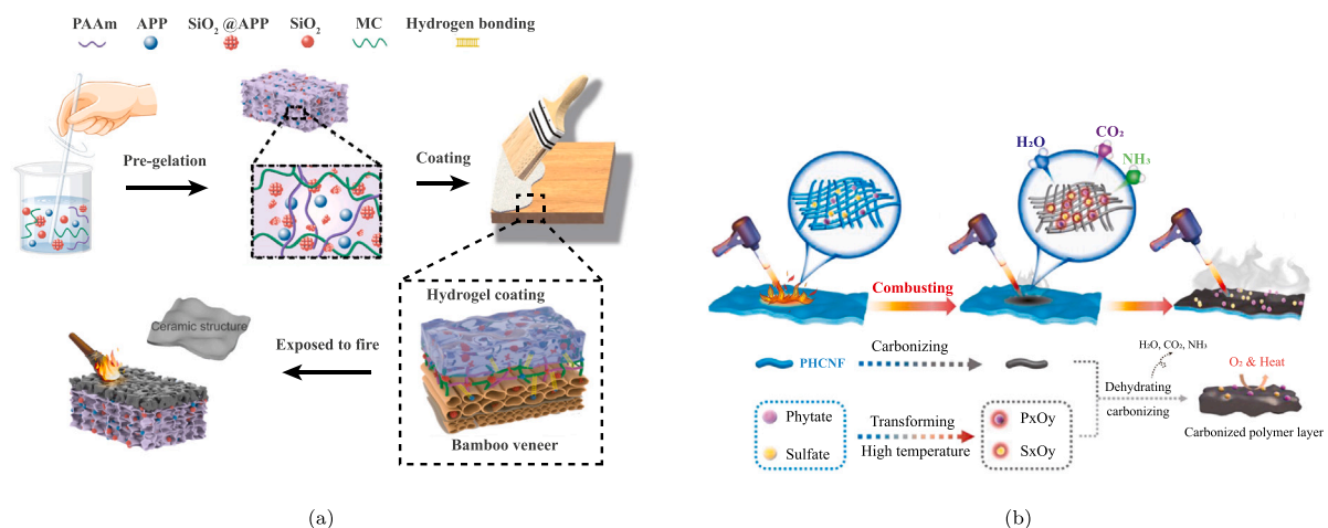
Fig. 40. (a) Schematic illustration of the flame-retardant function of the hydrogel coating. Adapted from Yu et al. [584]. (b) Flame-retardant mechanism of the PHCNF. Adapted from Ye et al. [588].
