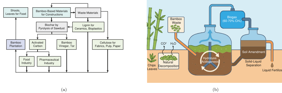
Fig. 41. (a) Reuse of bamboo material as part of the circular economy. Adapted from Yadav and Mathur [630]. (b) Typical anaerobic digestion process for biogas and organic fertiliser production from bamboo waste.
