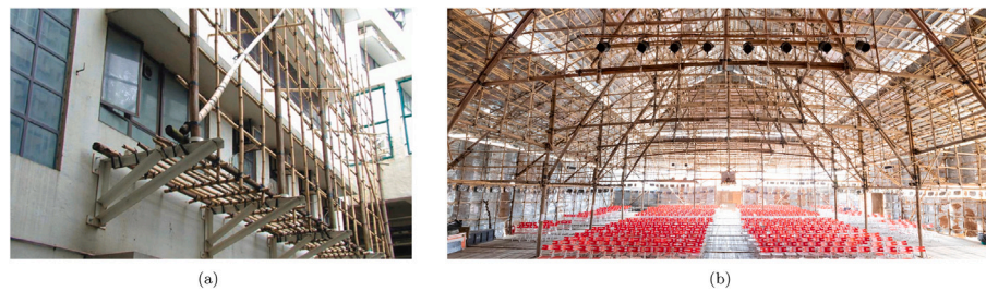
Fig. 27. (a) Steel bracket support for bamboo scaffolding. After Ramanathan [452]. (b) A bamboo theatre building in Hong Kong [453].
