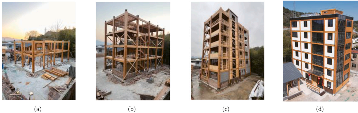
Fig. 35. The assembly construction process of the seven-story bamboo structure. (a) First and second floor construction unit; (b) third and fourth floor construction unit; (c) completed seven-story structural frame; and (d) completed building. Adapted from Wu et al. [486].
