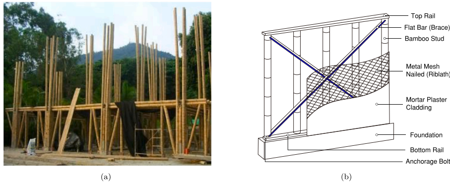
Fig. 18. Typical round bamboo member: (a) beam and column in framing system; (b) stud or brace in CBFT wall. Adapted from Archila-Santos et al. [283] and Bundi et al. [281], respectively.
